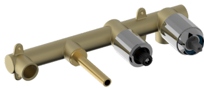
Corpo incasso universale per vasca Concealed body for bathtub mixer
