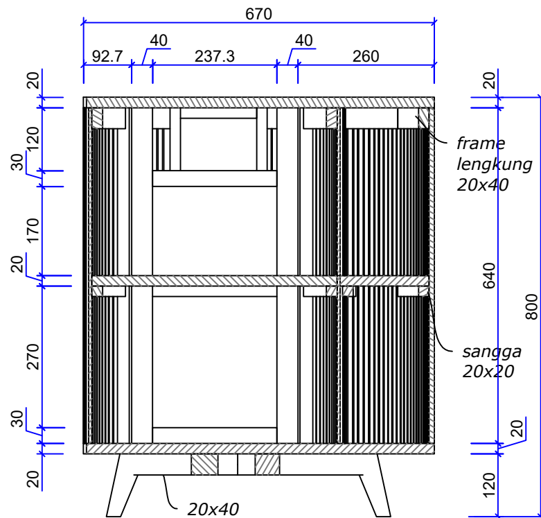
SECTION B-B
