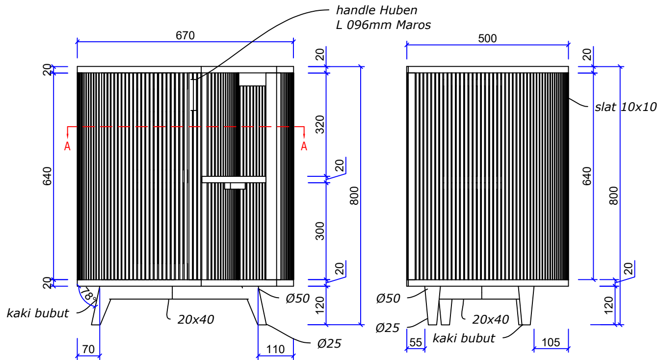
FRONT VIEW T. Depan
